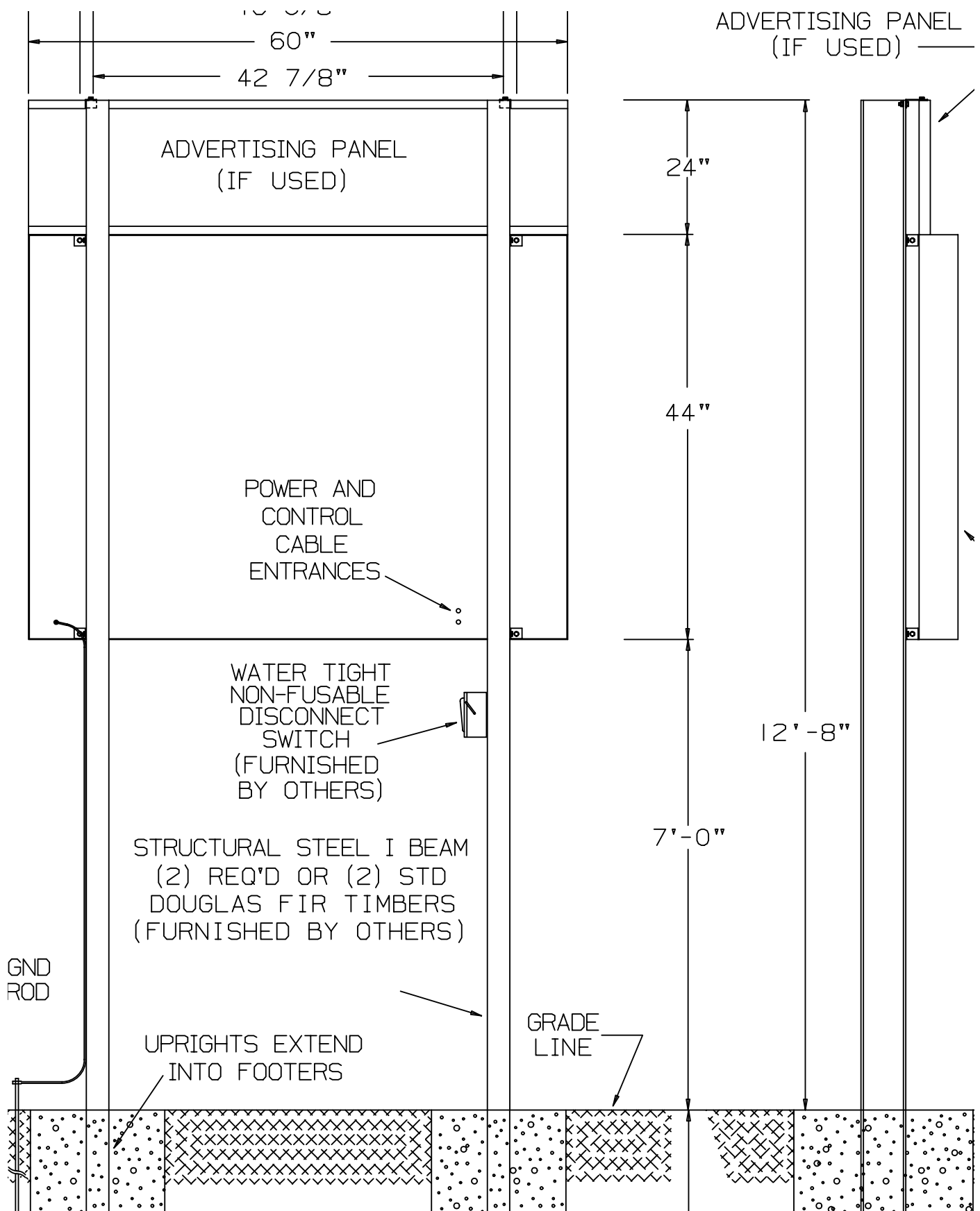
6.10 (cont.) Installation Drawing With Illuminated Ad. Panel
